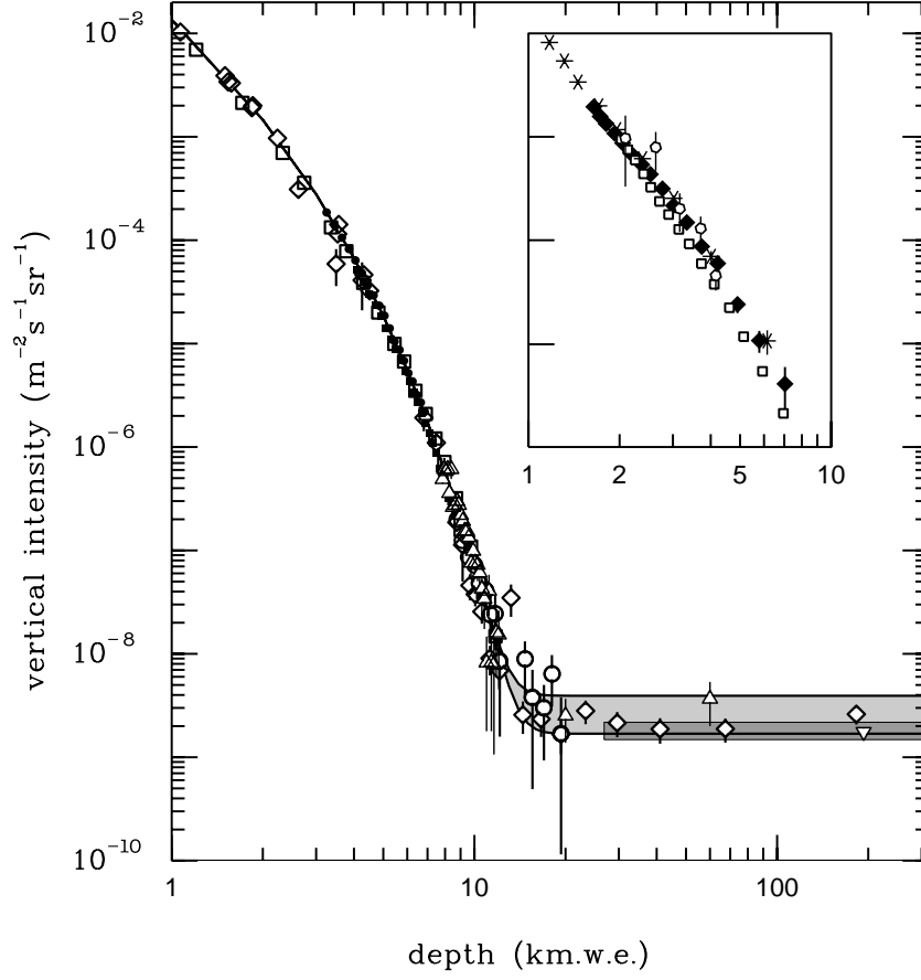
Figure 29.7: Vertical muon intensity vs depth (1 km.w.e. = 10^5 g cm ^{-2} of standard rock). The experimental data are from: \diamond : the compilations of Crouch [69], \square : Baksan [74], \circ : LVD [75], \bullet : MACRO [76], \blacksquare : Frejus [77], and \triangle : SNO [78]. The shaded area at large depths represents neutrino-induced muons of energy above 2 GeV. The upper line is for horizontal neutrino-induced muons, the lower one for vertically upward muons. Darker shading shows the muon flux measured by the SuperKamiokande experiment. The inset shows the vertical intensity curve for water and ice published in Refs. [70–73].
