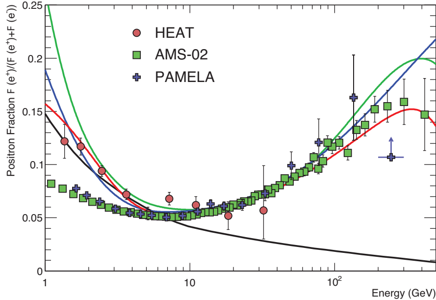
Figure 29.3: The positron fraction (ratio of the flux of e^+ to the total flux of e^+ and e^- ) [26,24,30]. The heavy black line is a model of pure secondary production [28] and the three thin lines show three representative attempts to model the positron excess with different phenomena: green: dark matter decay [29]; blue: propagation physics [32]; red: production in pulsars [40]. The ratio below 10 GeV is dependent on the polarity of the solar magnetic field.
