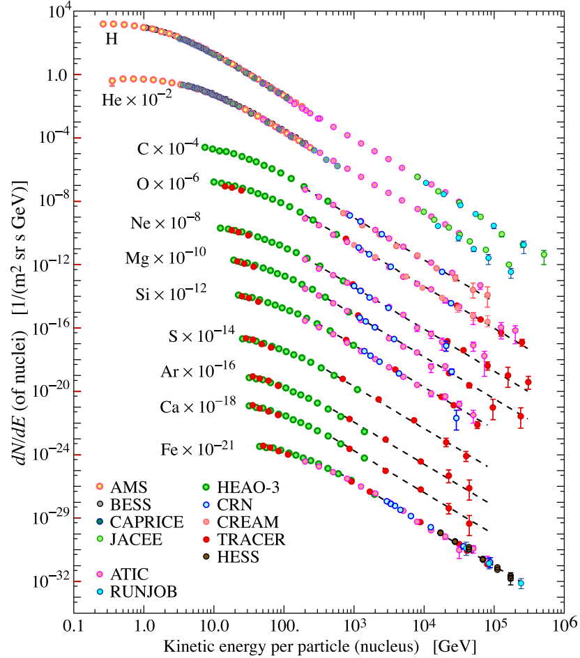
Figure 29.1: Fluxes of nuclei of the primary cosmic radiation in particles per energy-per-nucleus are plotted vs energy-per-nucleus using data from Refs. [2–13]. The figure was created by P. Boyle and D. Muller.
