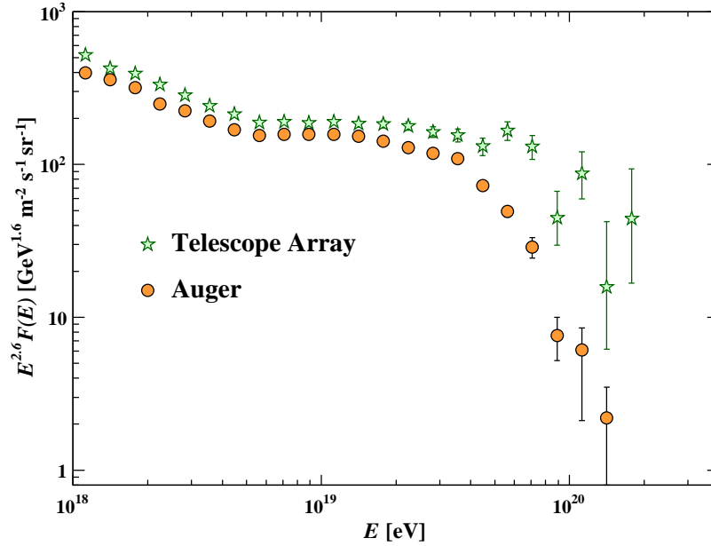
Figure 29.9: Expanded view of the highest energy portion of the cosmic-ray spectrum from data of the Telescope Array [104], and the Auger Observatory [105].
