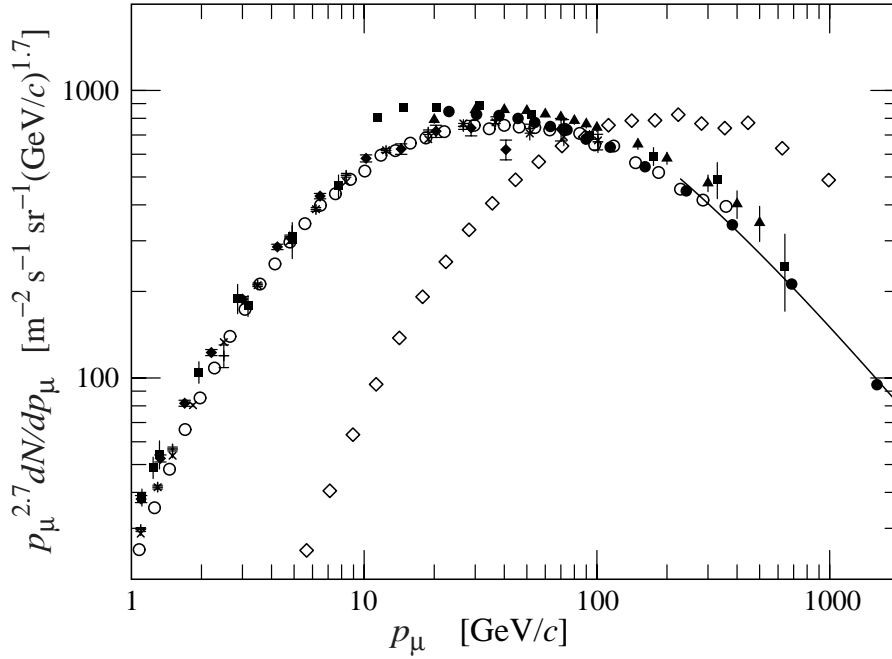
Figure 29.5: Spectrum of muons at \theta = 0^\circ ( \diamond [50], \blacksquare [56], \blacktriangledown [57], \blacktriangle [58], \times , + [52], \circ [53], and \bullet [54] and \theta = 75^\circ \diamond [59]). The line plots the result from Eq. (29.4) for vertical showers.
