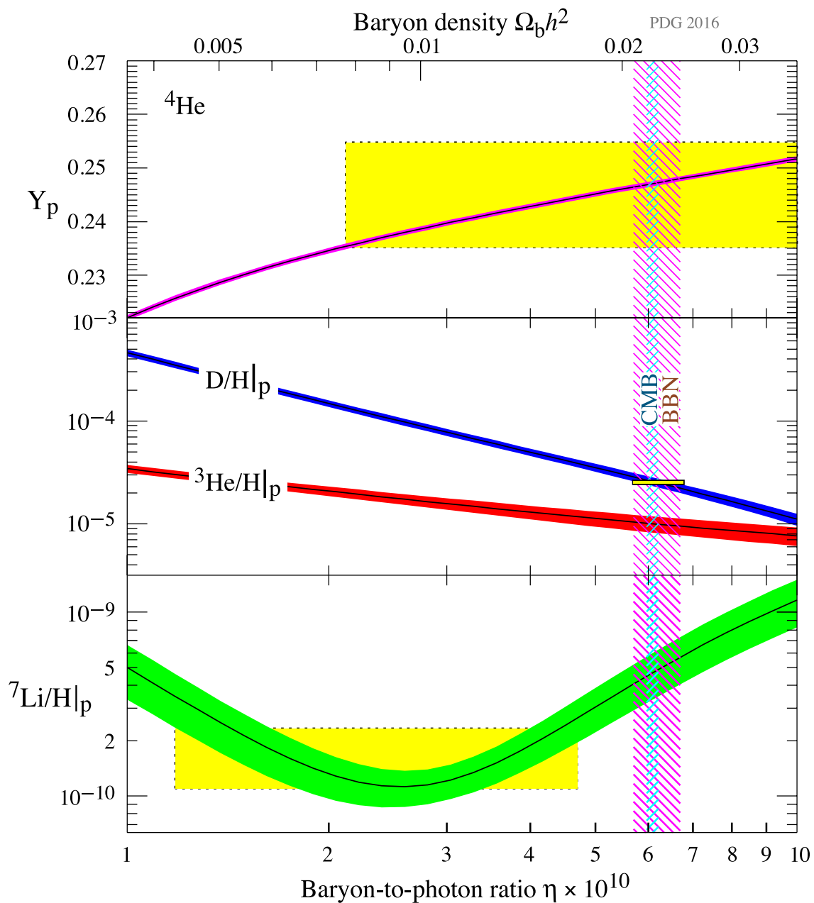
Figure 24.1: The primordial abundances of ^4\text{He} , D, ^3\text{He} , and ^7\text{Li} as predicted by the standard model of Big-Bang nucleosynthesis—the bands show the 95% CL range [5]. Boxes indicate the observed light element abundances. The narrow vertical band indicates the CMB measure of the cosmic baryon density, while the wider band indicates the BBN concordance range (both at 95% CL).
