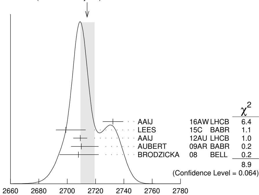
WEIGHTED AVERAGE 2714±5 (Error scaled by 1.5)
