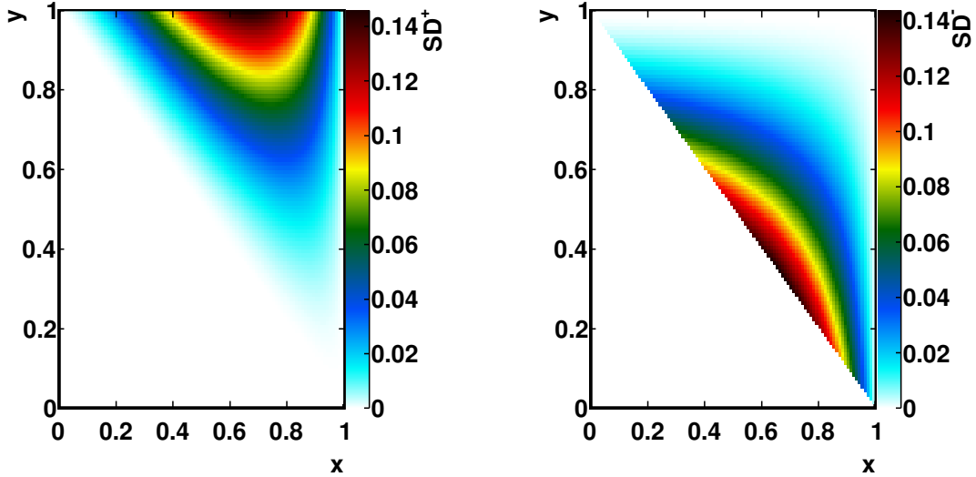
Figure 61.1: Components of the structure dependent terms of the decay width. Left: \text{SD}^+ , right: \text{SD}^-
